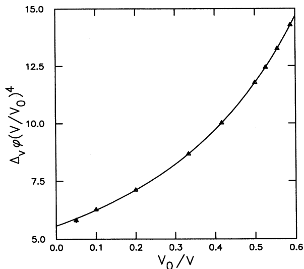
FIG. 3. Deviation \Delta_v \phi of the compressibility factor from the three-term virial series as a function of reduced density V_0/V . The curve is the [3/1] rational function fit, Eq. (9), to the data, with coefficients given by Eq. (10). Statistical uncertainties are marked at plus or minus one standard deviation.
