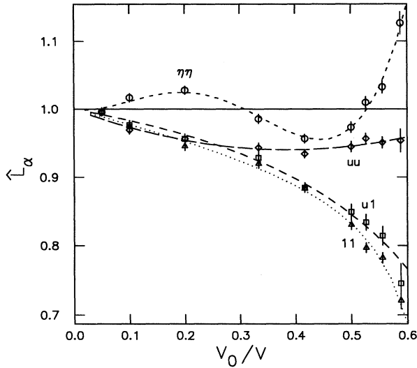
FIG. 4. Transport coefficients relative to the Enskog values \hat{L}_\alpha as functions of reduced density V_0/V : \alpha=11 for the mutual diffusion, \alpha=u1 for the thermal diffusion, \alpha=uu for the heat conductivity, and \alpha=\eta\eta for the shear viscosity. The lines are rational function fits, Eq. (15). Statistical uncertainties are marked with plus or minus one standard deviation.
