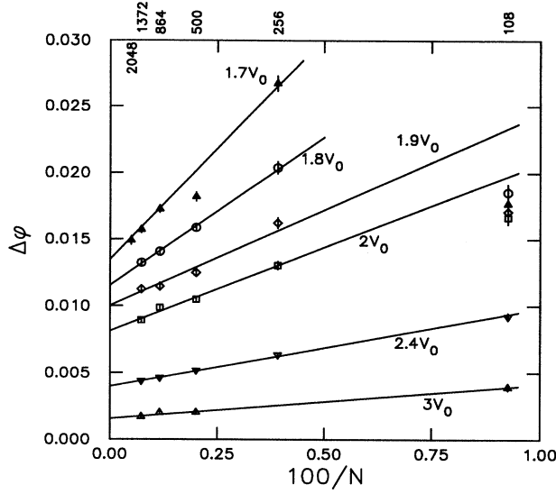
FIG. 1. Deviation \Delta\phi of the reduced pressure pV_0/Nk_B T from the MCSL prediction as a function of the number N of particles at volumes of 3V_0 (triangle, point up), 2.4V_0 (triangle, point down), 2V_0 (square), 1.9V_0 (diamond), 1.8V_0 (circle), and 1.7V_0 (filled triangle). The lines are weighted least-square fits to the N > 500 data for 1.7V_0 , the N \geq 256 data for 1.8V_0 \leq V \leq 2V_0 , and to all values of N for V \geq 2.4V_0 . Statistical uncertainties are marked at plus or minus one standard deviation.
