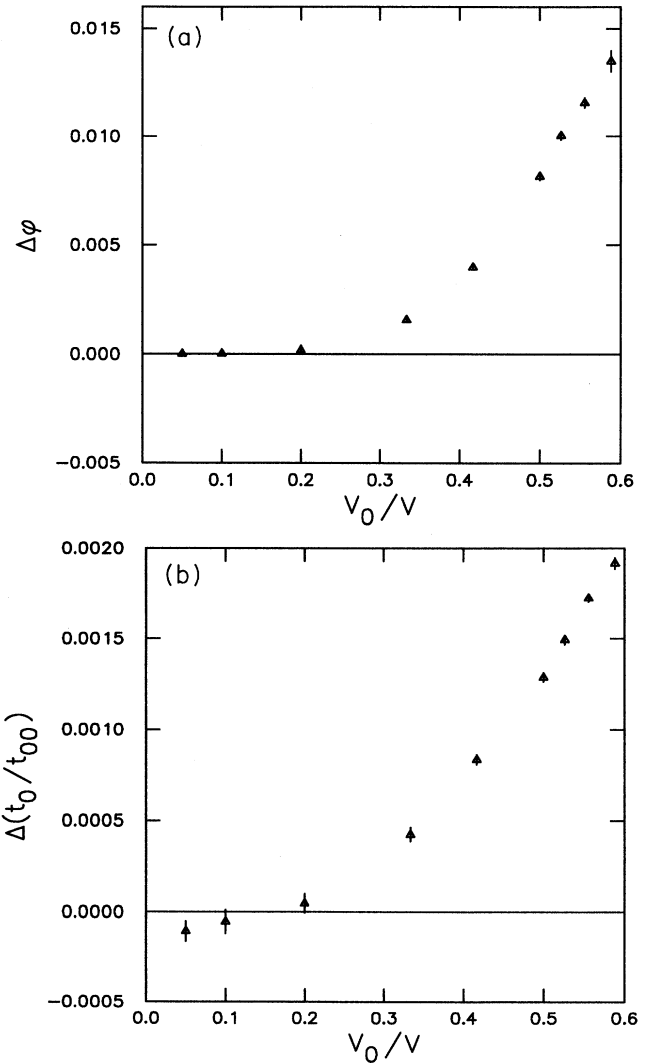
FIG. 2. Deviation of the equation of state from the MCSL equation of state as a function of reduced density V_0/V : (a) the reduced pressure \phi and (b) the mean free time t_0 relative to the Boltzmann value t_{00} . Statistical uncertainties are marked at plus or minus one standard deviation.
